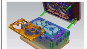
Mold Design
